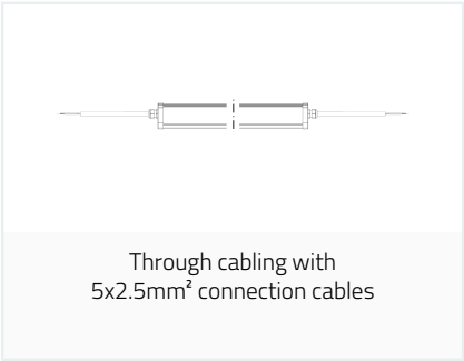
Through cabling with 5x2.5mm 2 Wago Winsta male connection cable at the other end and integrated female connector at the other end of the luminaire.
